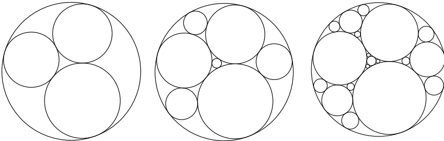
Figure 1. An Apollonian circle packing.
