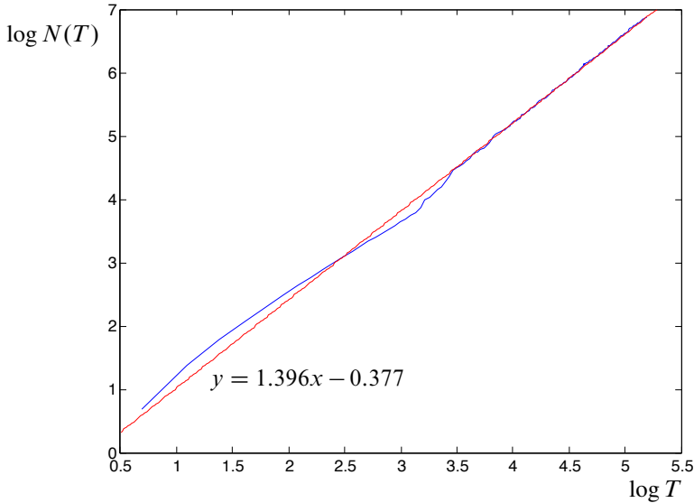
Figure 2. Counting elements in a symplectic monodromy group.
