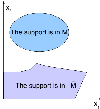
Figure 1. The support of an element of C_0^\infty(\Lambda^k M) and the support of an element of C_0^\infty(\Lambda^k \overline{M}) . Here \overline{M} is the positive quadrant \{x_1 \geq 0, x_2 \geq 0\} in the plane.
