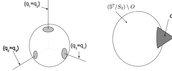
Figure 2. Left: The three collision planes in (\mathbb{C}^2)^3_0 . Right: \mathbb{S}^7/S_3 .
