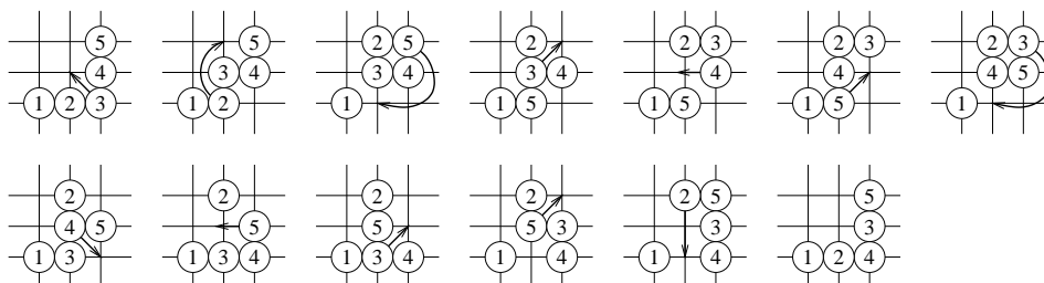
Figure 31. Solution to the puzzle in Figure 8.
