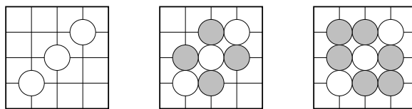
Figure 18. In this example, the span is the smallest rectangle enclosing the configuration.
