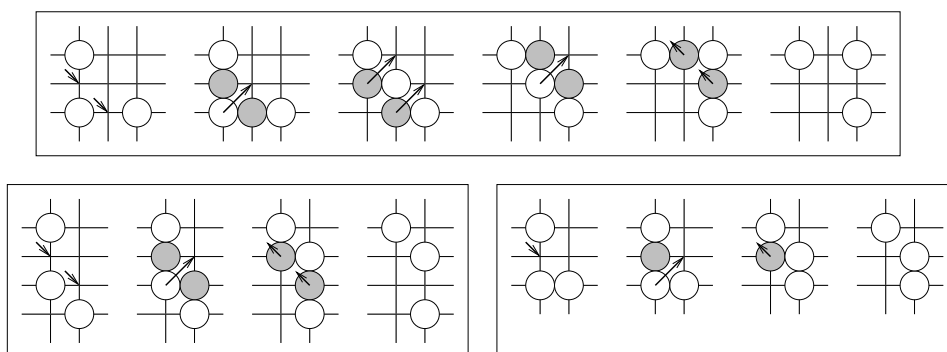
Figure 23. Flipping an L consisting of 3 coins. Extra coins are shaded.
