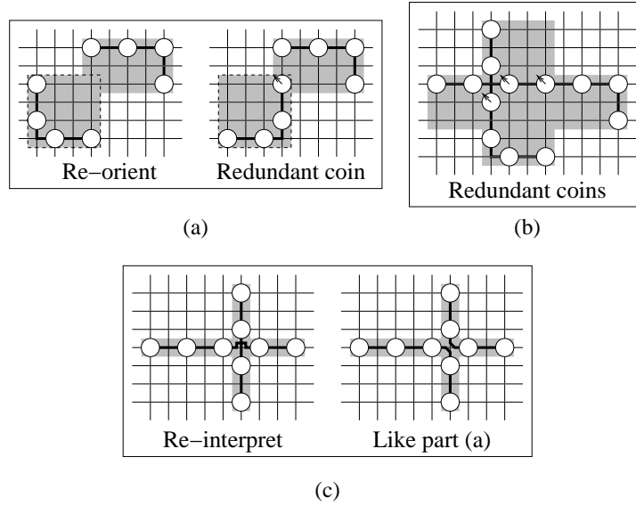
Figure 27. Merging two L's with overlapping bounding rectangles (shaded). (a) The corner of one L is contained in the other L's bounding rectangle. (b) A "thick plus sign" in which at least one stroke has thickness more than 1. (c) A plus sign in which both strokes have thickness 1.
