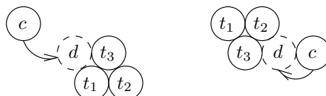
Figure 14. Transporting coin c to destination d using triangle \{t_1, t_2, t_3\} . In both cases, we choose the location of the triangle so that it does not overlap c .
