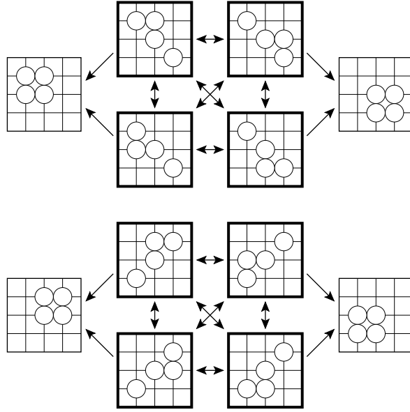
Figure 20. Subgraph of configuration space reachable from full-span configurations (outlined in bold) with one extra token.
