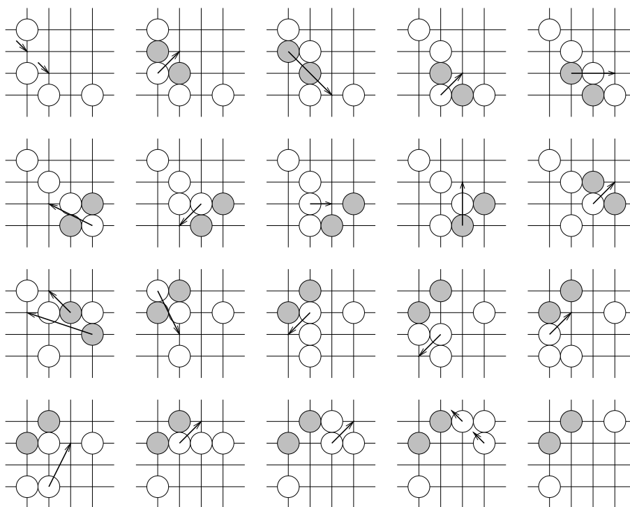
Figure 25. One method for rotating an L with a square span. Although this example places the extra coins in the final configuration, this is not necessary.
