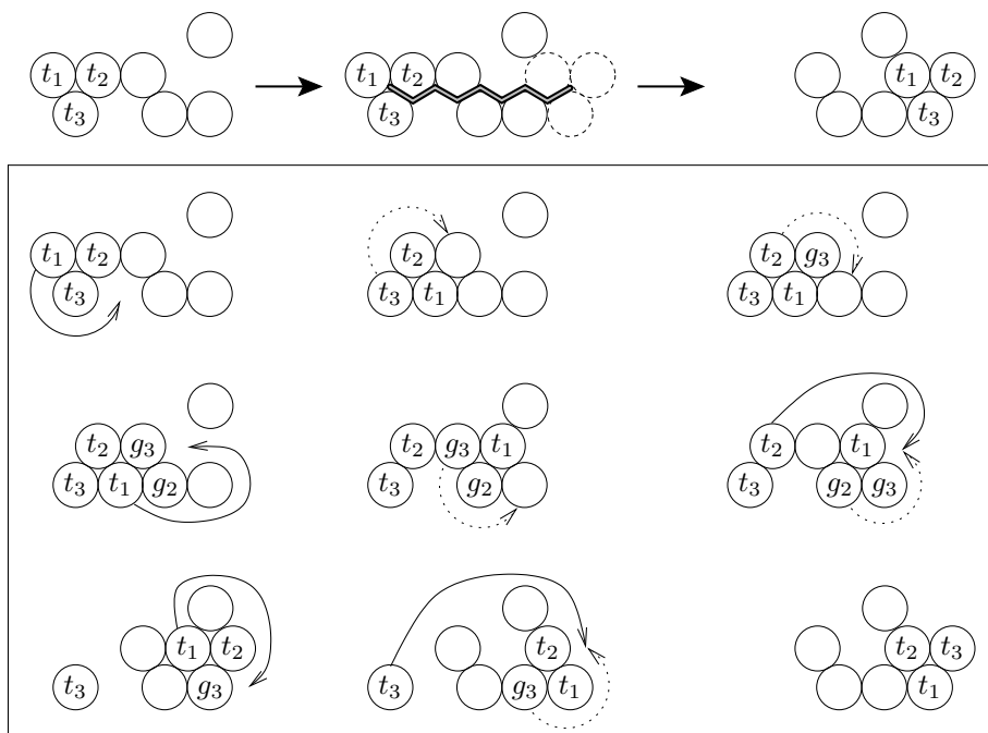
Figure 13. An example of triangle maneuvering. Dotted arrows denote conceptual moves, and solid arrows denote actual moves.
