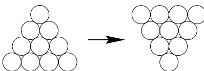
Figure 2. Turn the pyramid upside-down in three moves, such that each coin is moved to a position adjacent to two other coins.
