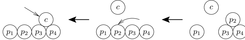
Figure 16. Reverse moving a configuration B with Property 2 into a configuration with Property 1.
