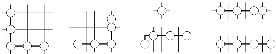
Figure 21. Examples of L 's.
