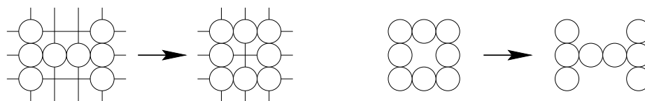
Figure 4. Re-arrange the H into the O in four moves while staying on the square grid (and always moving adjacent to two other coins), and return to the H in six moves using both the equilateral-triangle and square grids.
