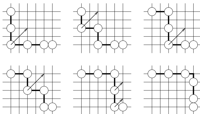
Figure 24. Flipping a general L, using the subroutines in Figure 23.
