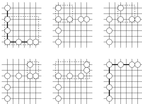
Figure 26. A general method for rotating an L. The first step is to apply induction, and the remaining steps apply subroutines similar to Figure 23.
