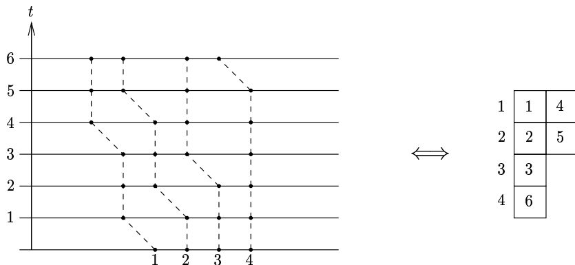
Figure 2. Random turn vicious walkers and Young tableaux.
