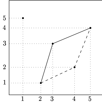
Figure 1. Random points in a rectangle.
